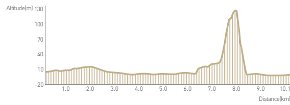
Elevation of Route #21
